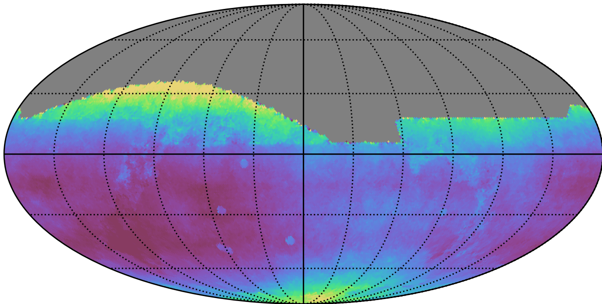
roman_v3.3_10yrs All sky all bands: Median seeingEff
