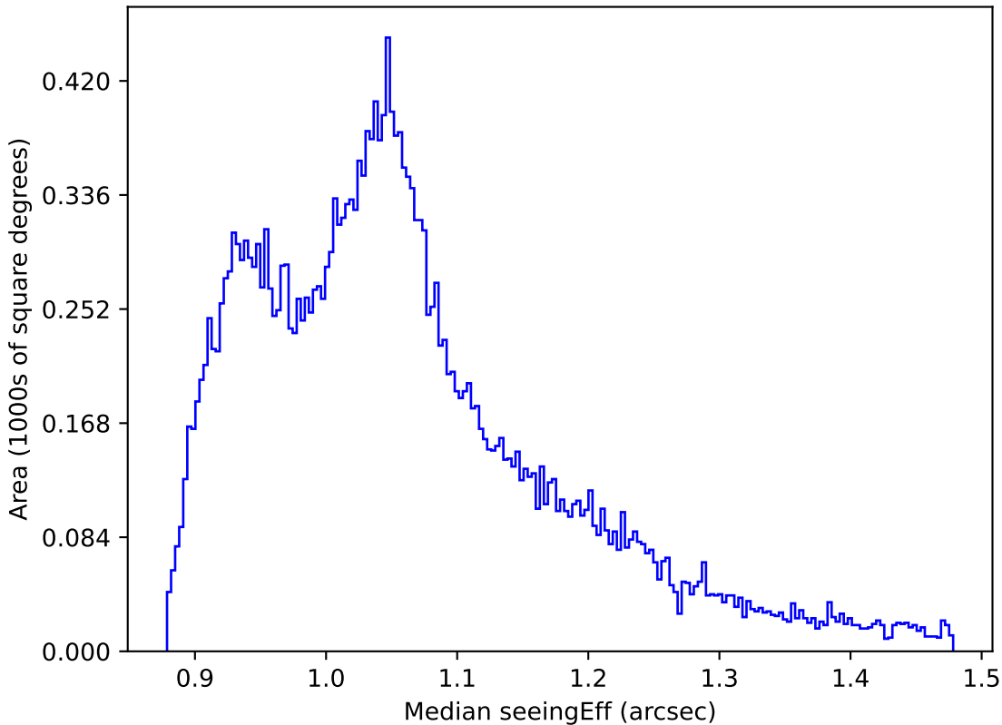
roman_v3.3_10yrs All sky all bands: Median seeingEff
