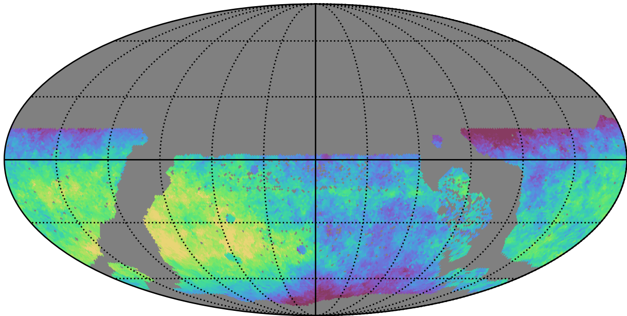
roman_v3.3_10yrs WFD z band: Median saturation_mag
