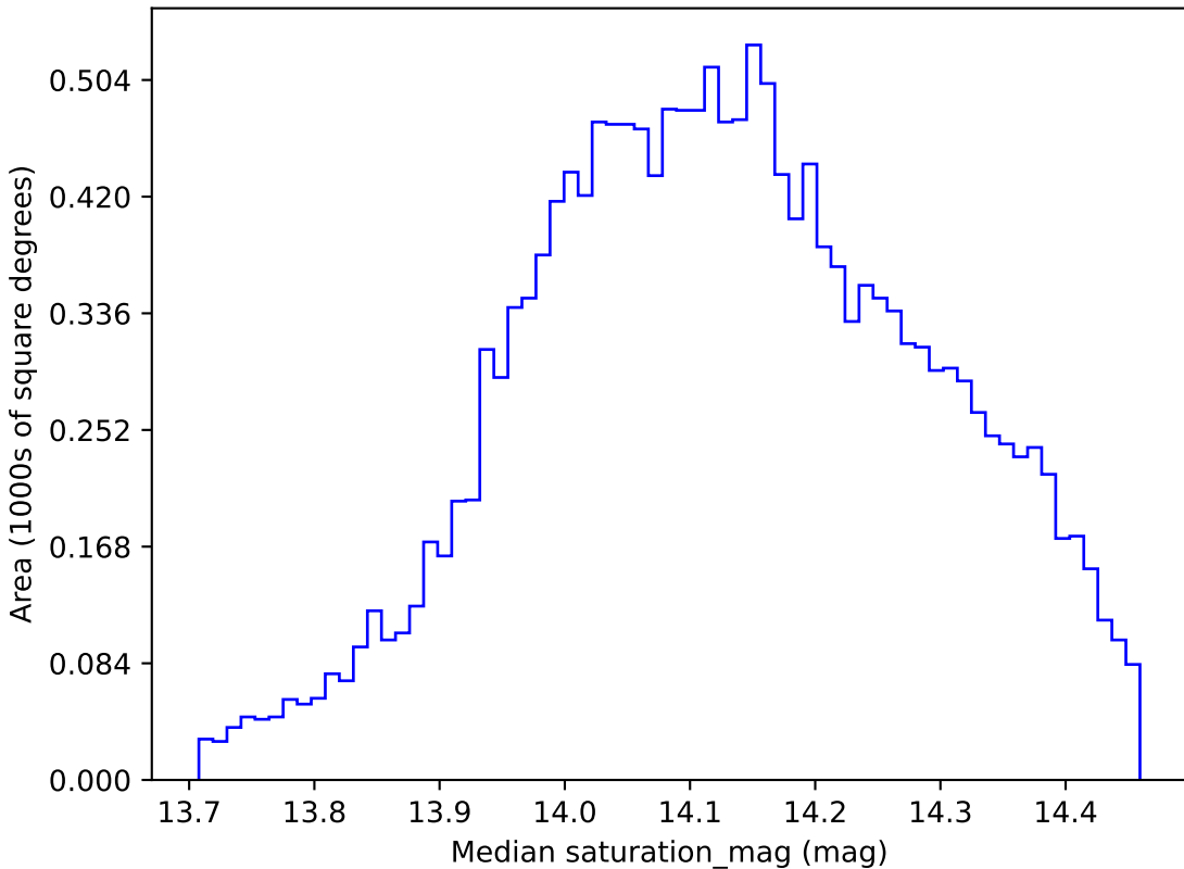
roman_v3.3_10yrs WFD z band: Median saturation_mag
