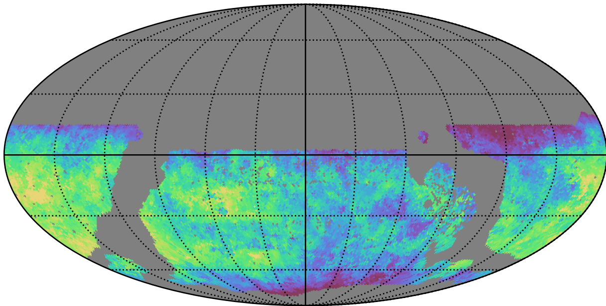
roman_v3.3_10yrs WFD u band: Median saturation_mag
