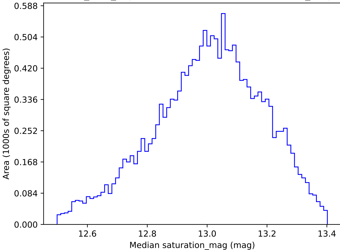
roman_v3.3_10yrs WFD u band: Median saturation_mag
