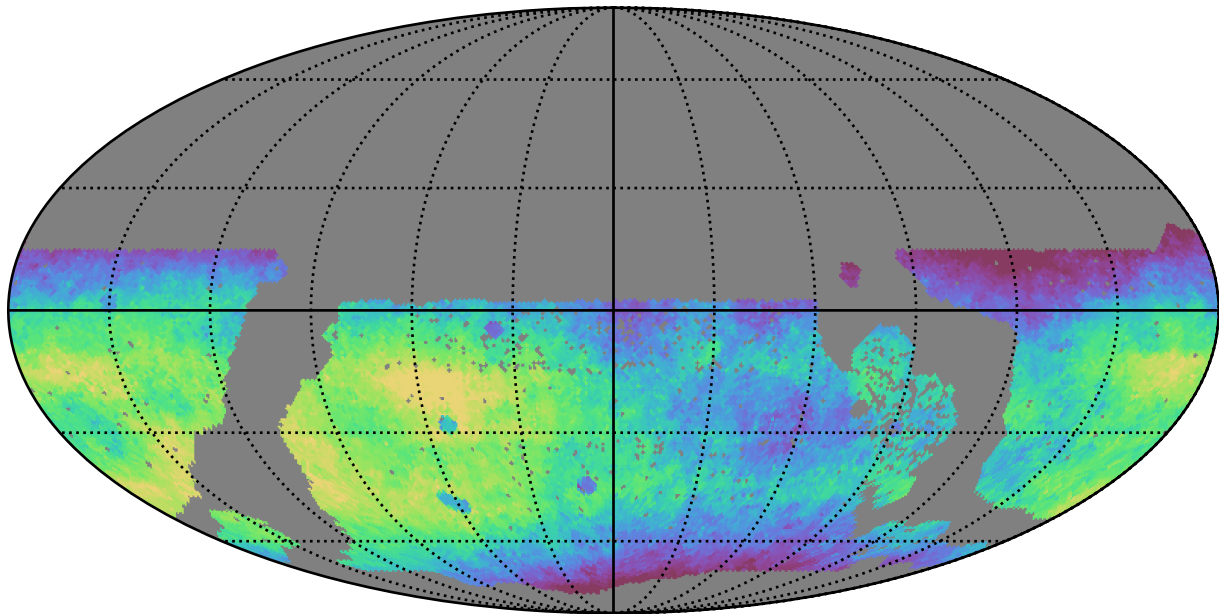
roman_v3.3_10yrs WFD r band: Median saturation_mag
