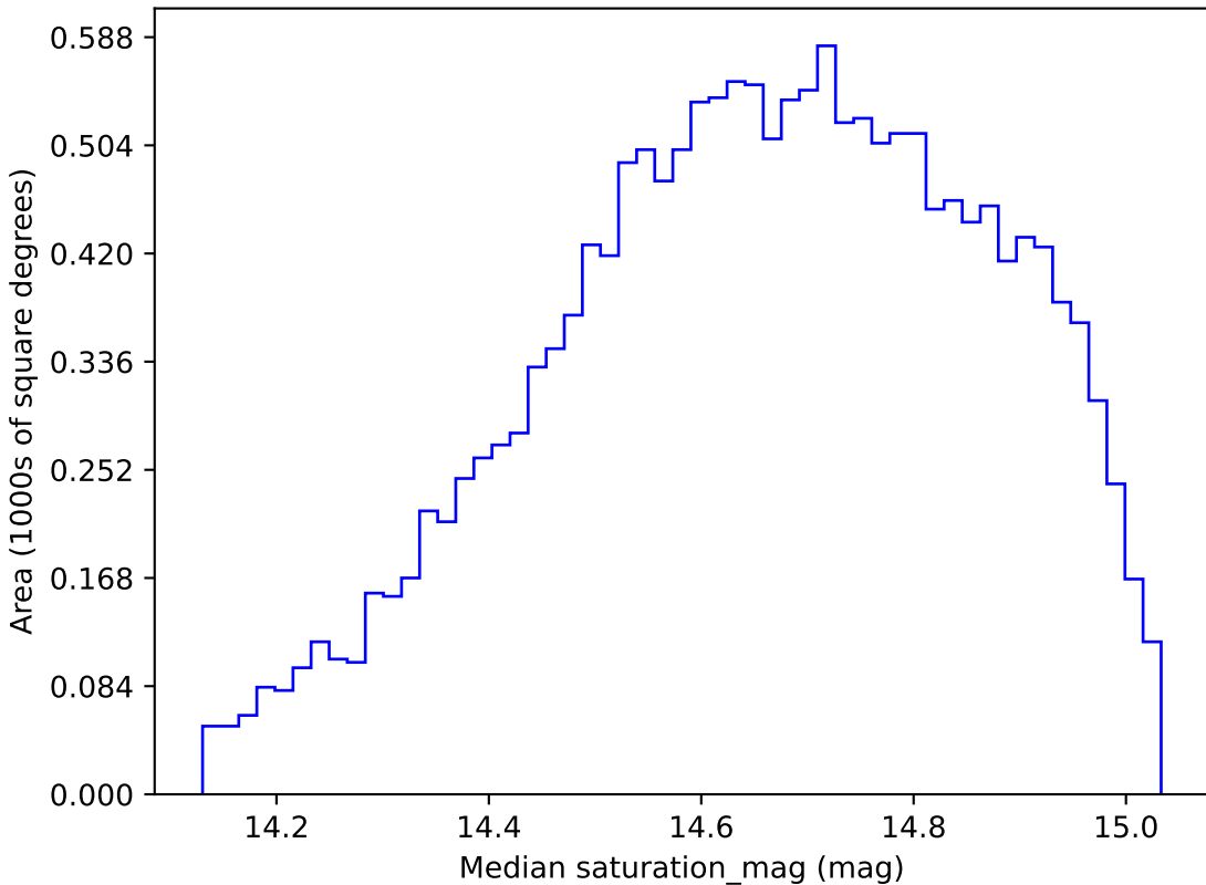
roman_v3.3_10yrs WFD r band: Median saturation_mag
