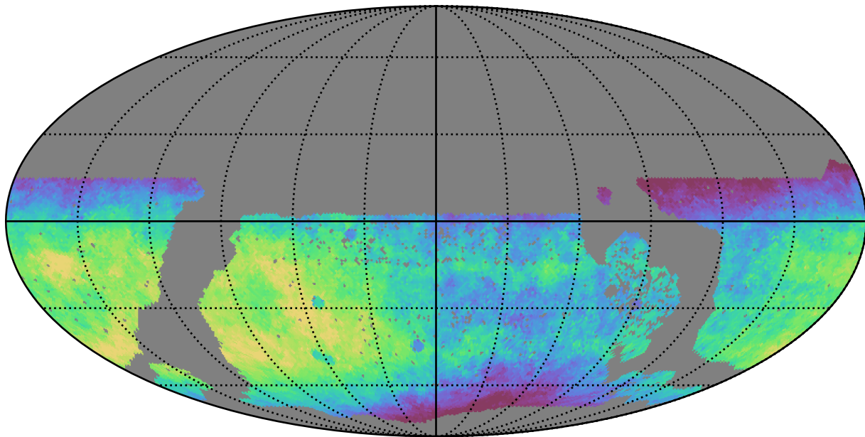
roman_v3.3_10yrs WFD i band: Median saturation_mag
