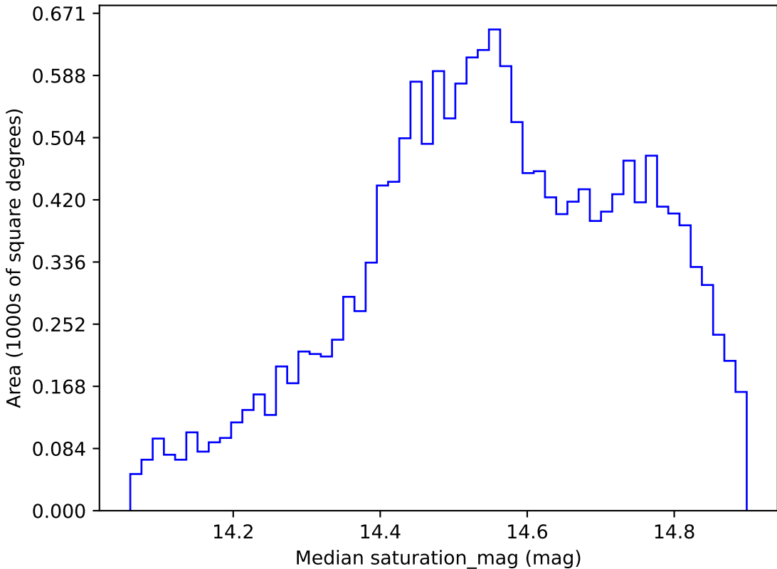
roman_v3.3_10yrs WFD i band: Median saturation_mag
