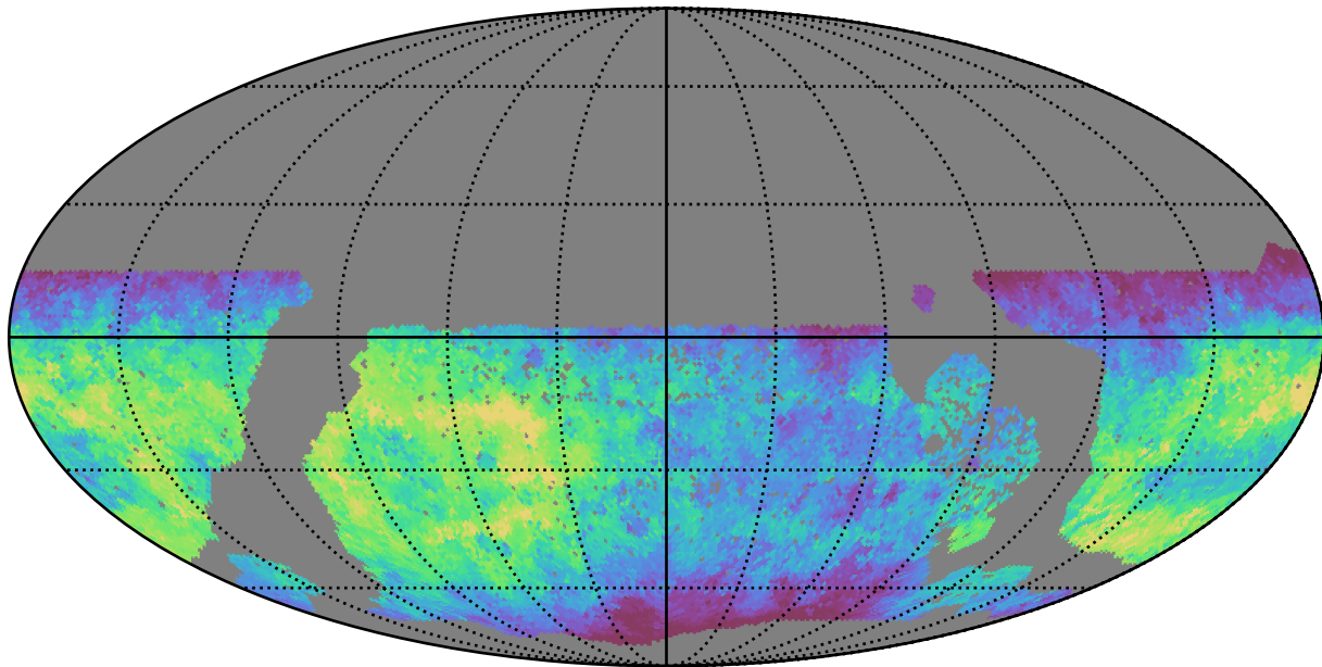
roman_v3.3_10yrs WFD g band: Median saturation_mag
