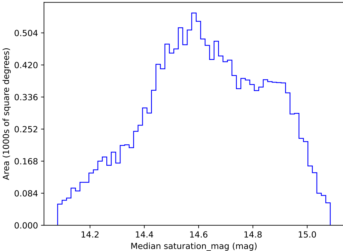
roman_v3.3_10yrs WFD g band: Median saturation_mag
