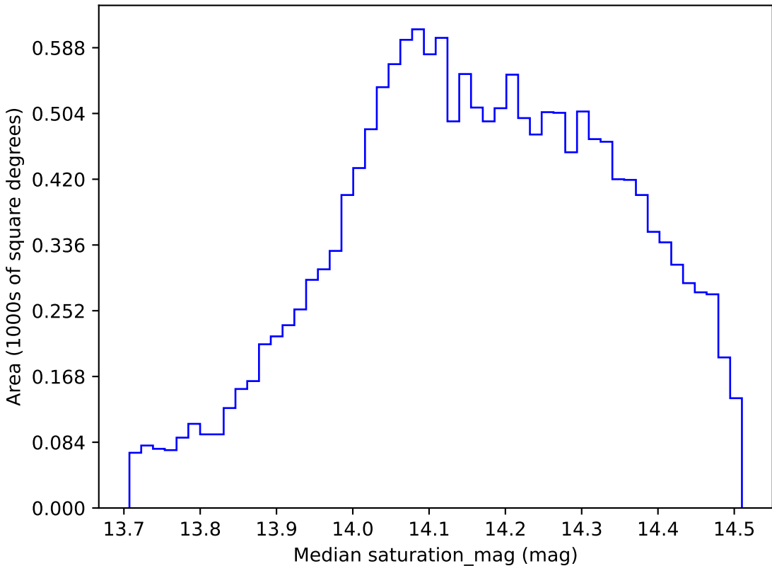
roman_v3.3_10yrs WFD all bands: Median saturation_mag
