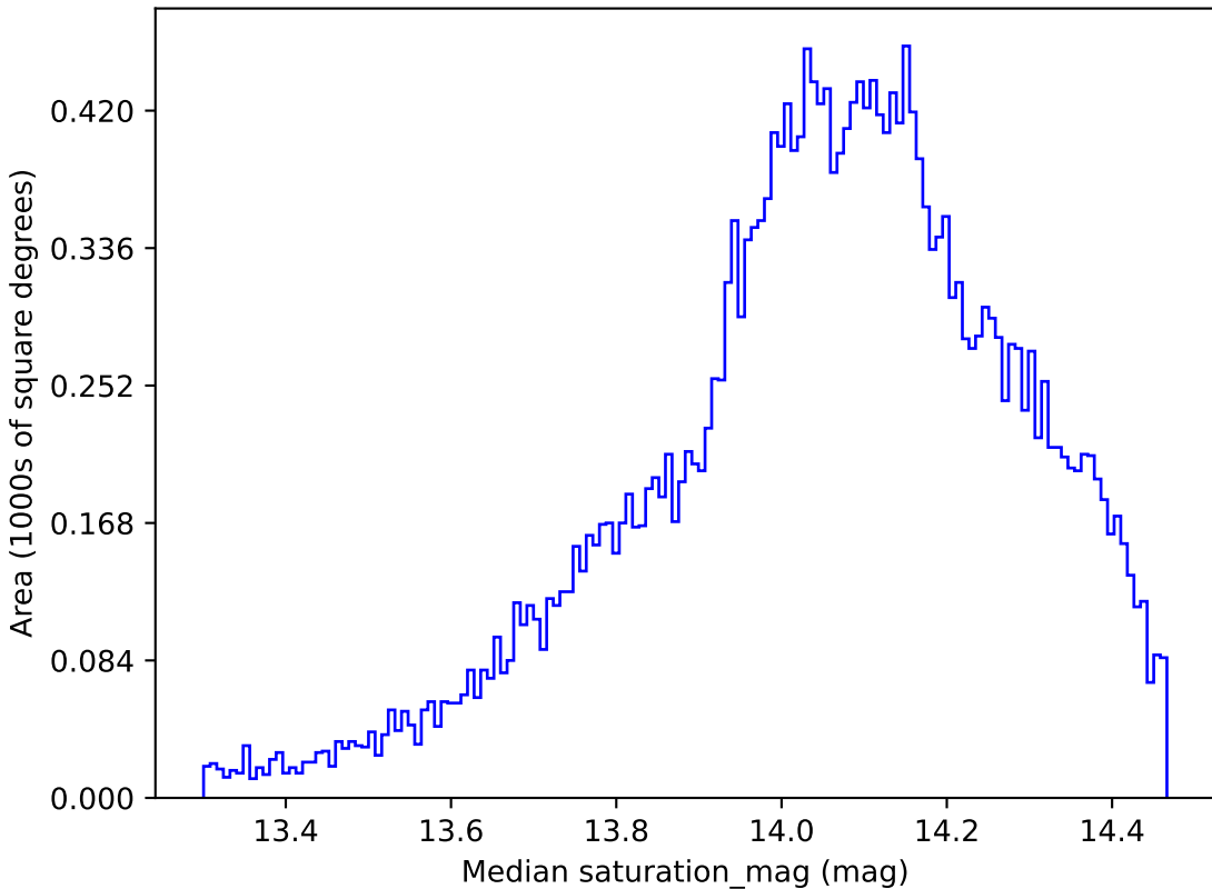
roman_v3.3_10yrs All sky z band: Median saturation_mag
