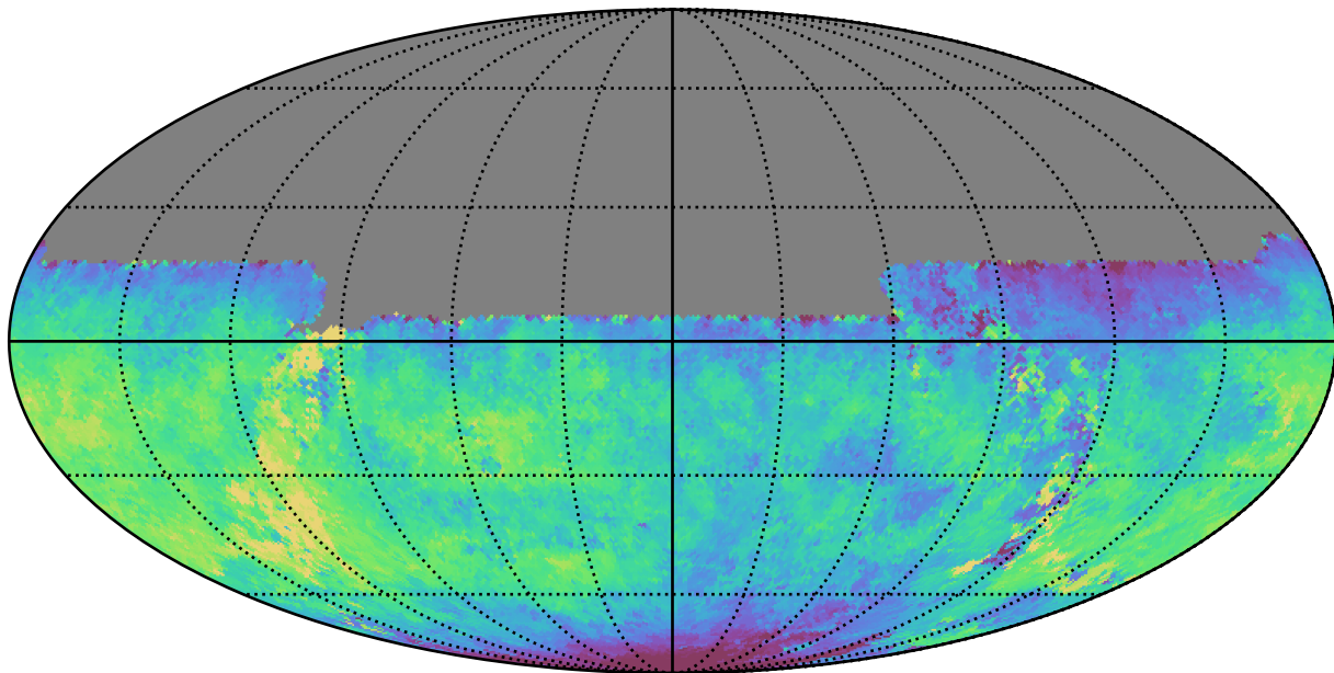
roman_v3.3_10yrs All sky u band: Median saturation_mag
