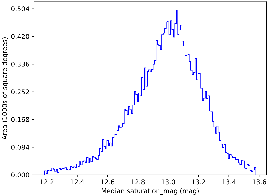
roman_v3.3_10yrs All sky u band: Median saturation_mag
