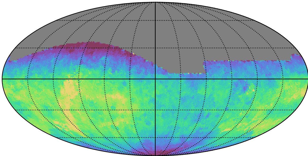
roman_v3.3_10yrs All sky g band: Median saturation_mag
