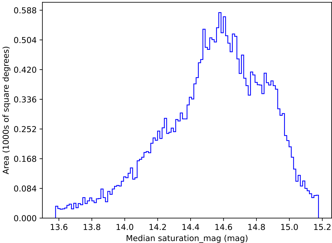
roman_v3.3_10yrs All sky g band: Median saturation_mag
