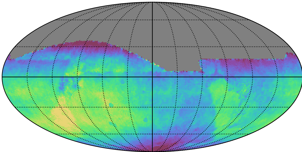
roman_v3.3_10yrs All sky all bands: Median saturation_mag
