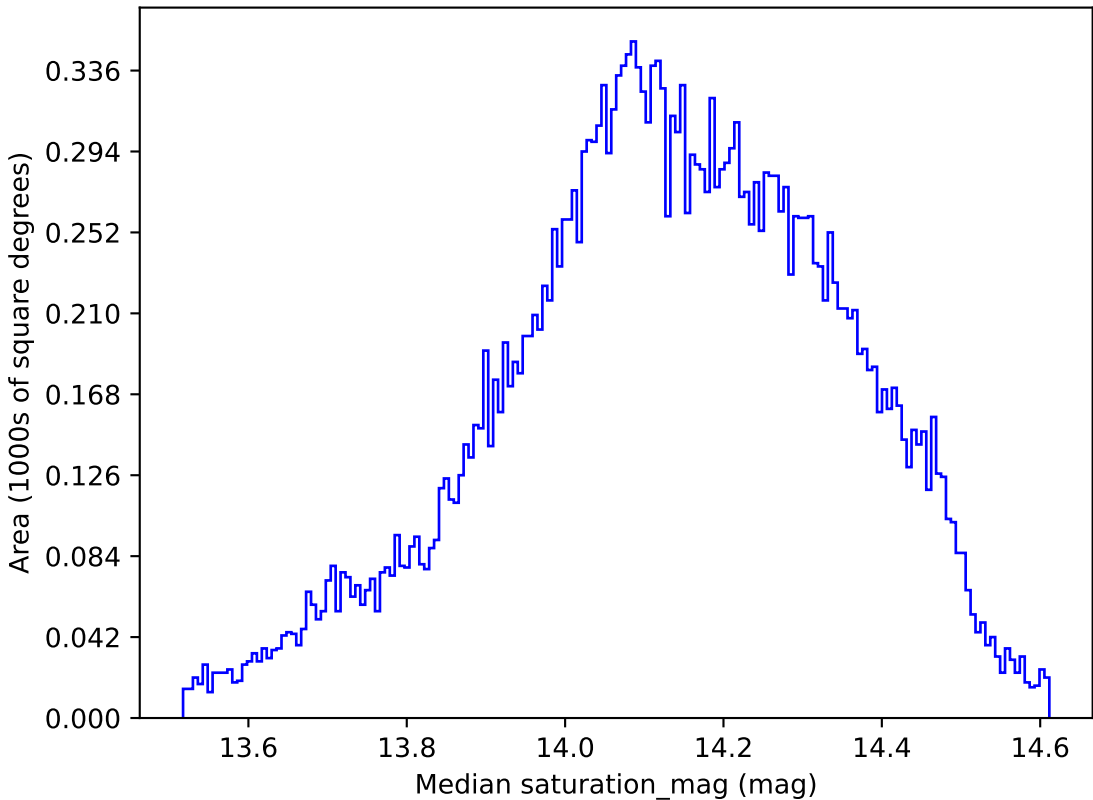
roman_v3.3_10yrs All sky all bands: Median saturation_mag
