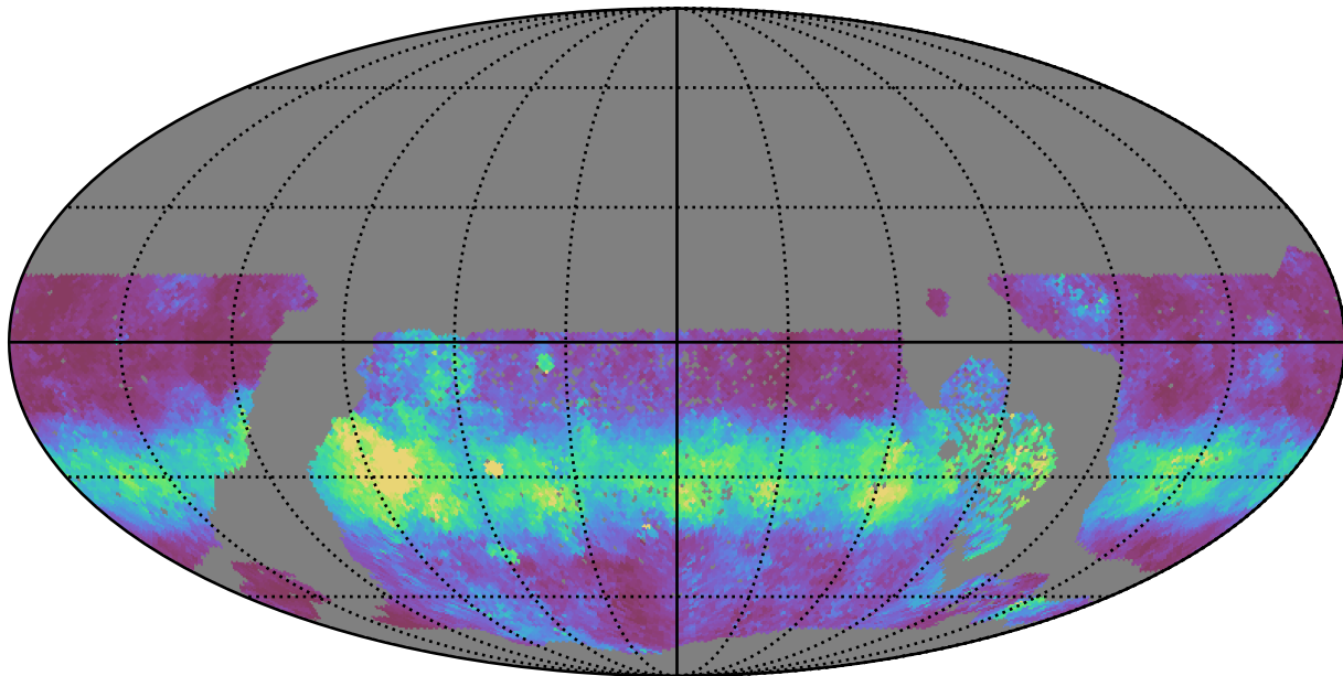
roman_v3.3_10yrs WFD u band: Median normairmass
