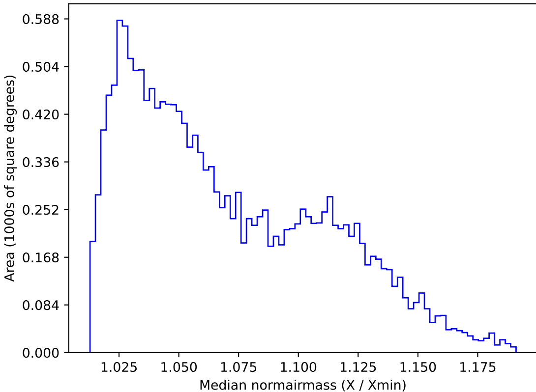
roman_v3.3_10yrs WFD u band: Median normairmass
