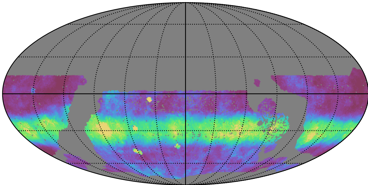
roman_v3.3_10yrs WFD r band: Median normairmass
