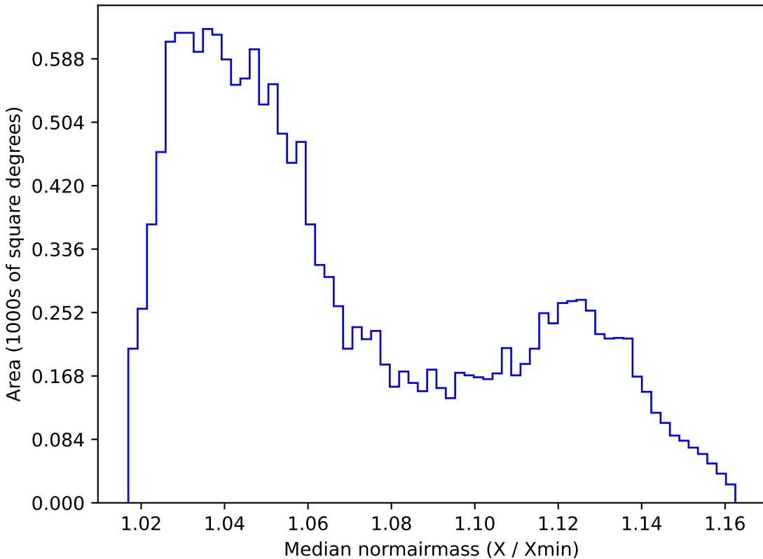
roman_v3.3_10yrs WFD r band: Median normairmass
