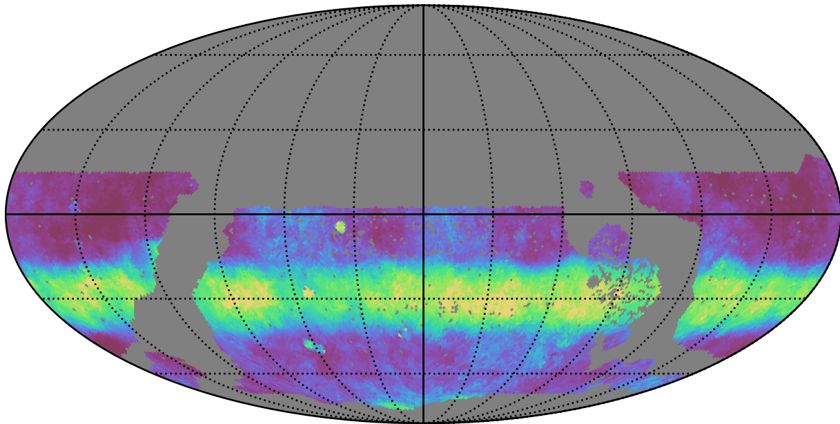
roman_v3.3_10yrs WFD i band: Median normairmass
