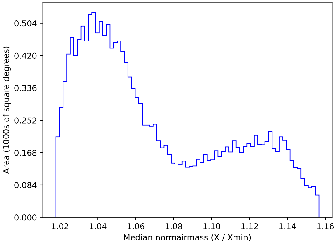
roman_v3.3_10yrs WFD i band: Median normairmass
