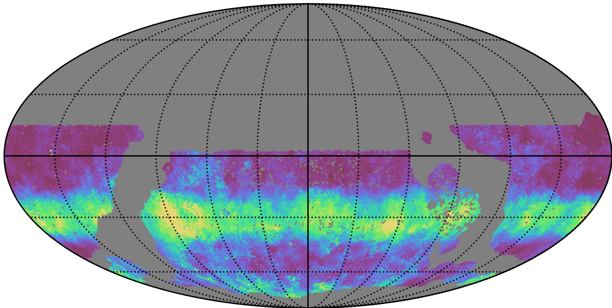
roman_v3.3_10yrs WFD g band: Median normairmass
