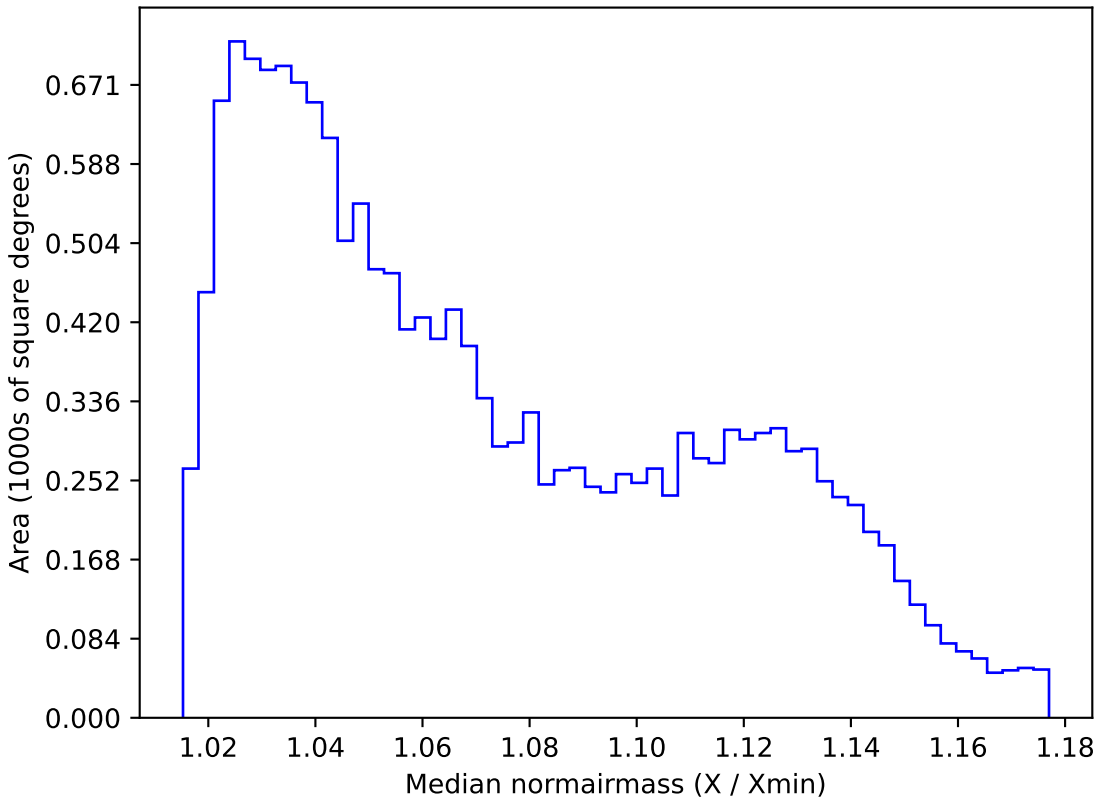
roman_v3.3_10yrs WFD g band: Median normairmass
