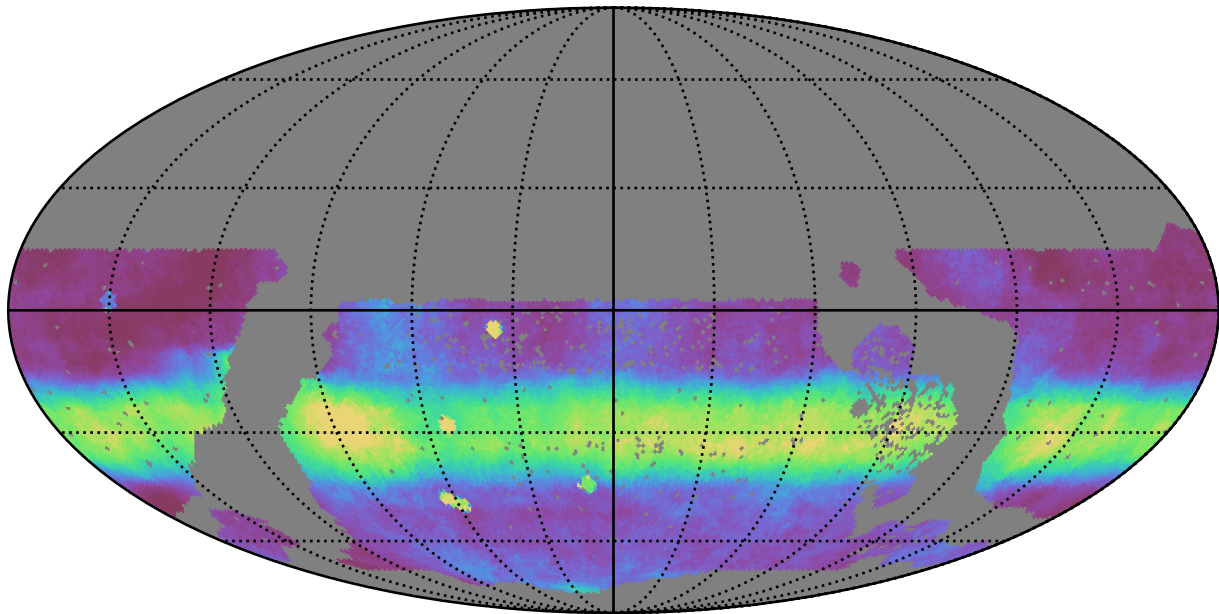
roman_v3.3_10yrs WFD all bands: Median normairmass
