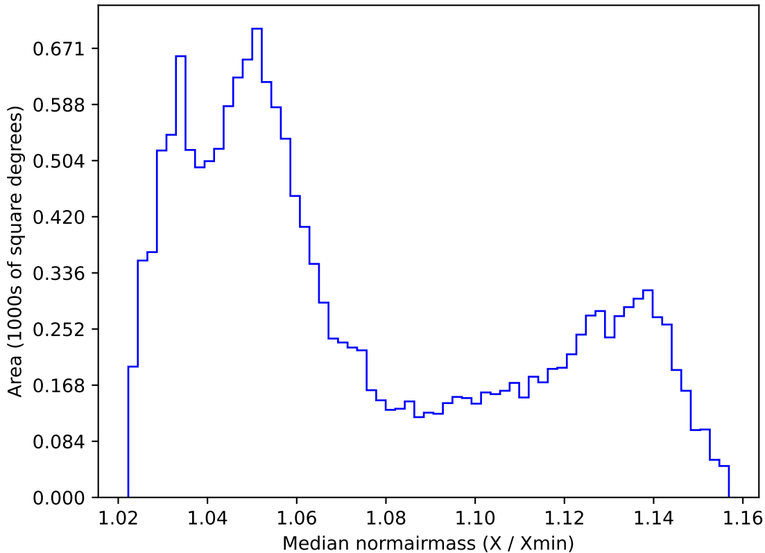
roman_v3.3_10yrs WFD all bands: Median normairmass
