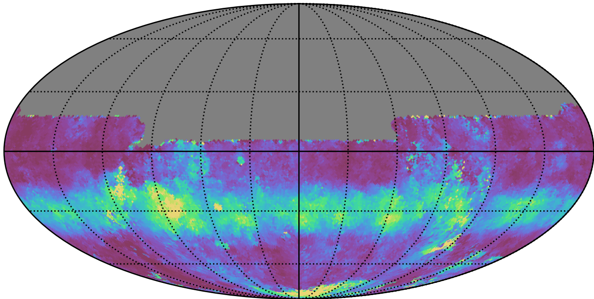
roman_v3.3_10yrs All sky u band: Median normairmass
