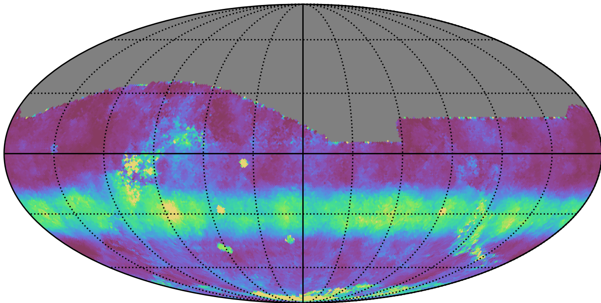
roman_v3.3_10yrs All sky r band: Median normairmass
