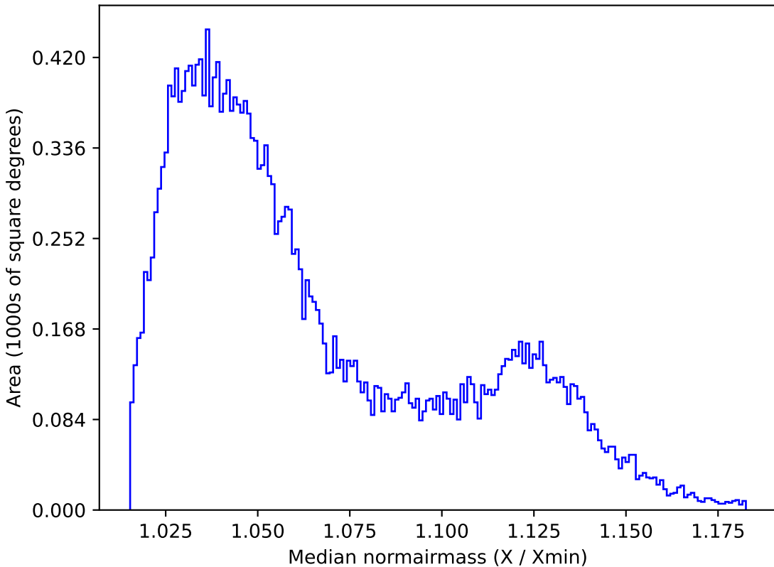
roman_v3.3_10yrs All sky r band: Median normairmass
