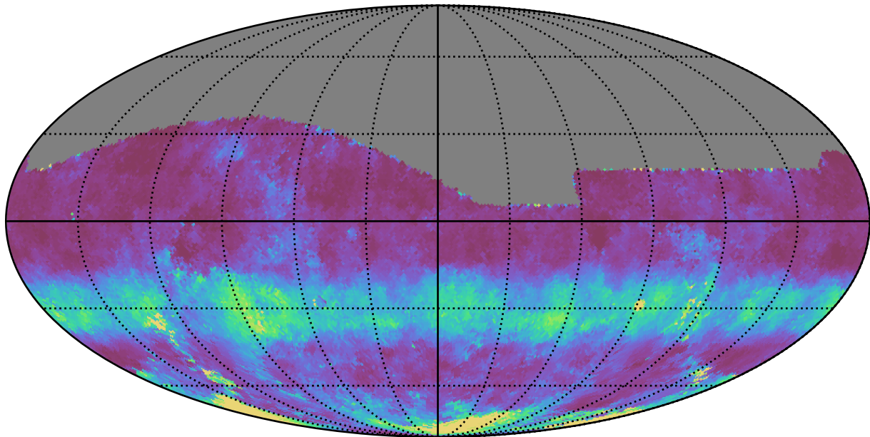
roman_v3.3_10yrs All sky g band: Median normairmass
