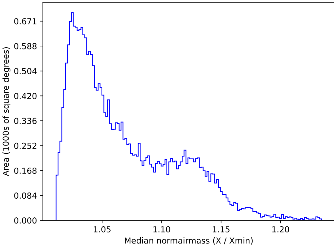
roman_v3.3_10yrs All sky g band: Median normairmass
