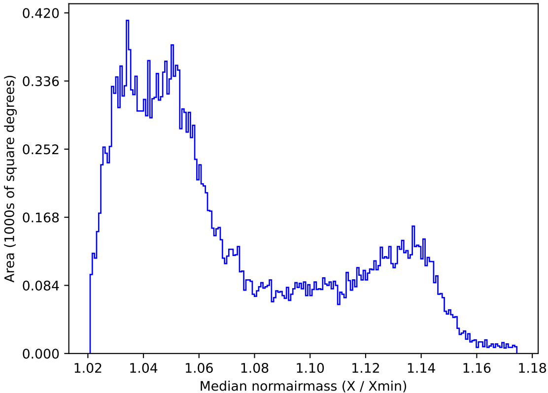
roman_v3.3_10yrs All sky all bands: Median normairmass
