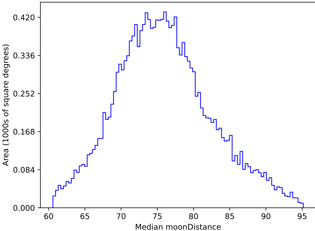
roman_v3.3_10yrs WFD z band: Median moonDistance
