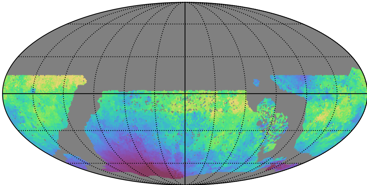
roman_v3.3_10yrs WFD u band: Median moonDistance
