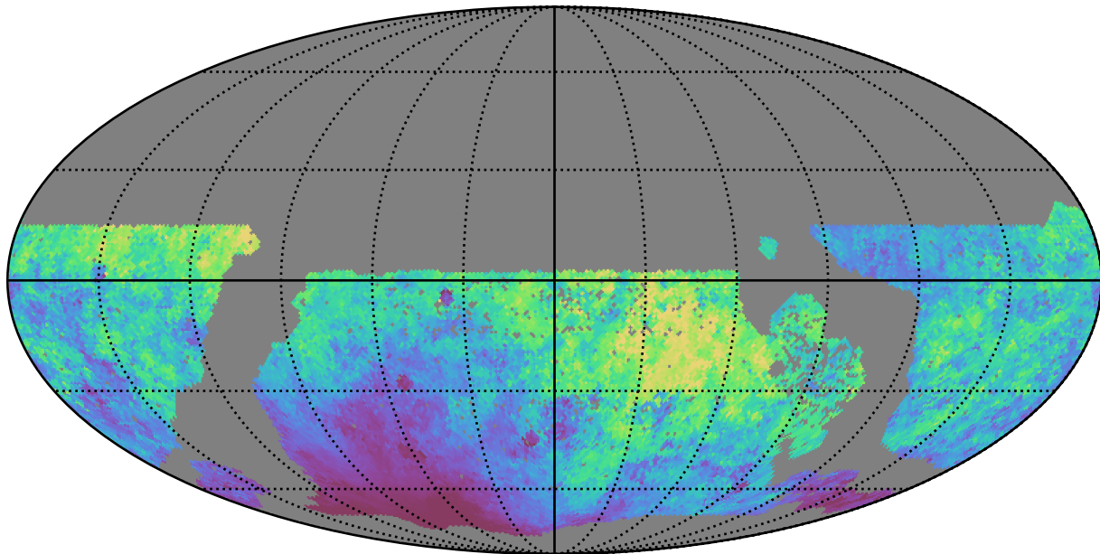
roman_v3.3_10yrs WFD r band: Median moonDistance
