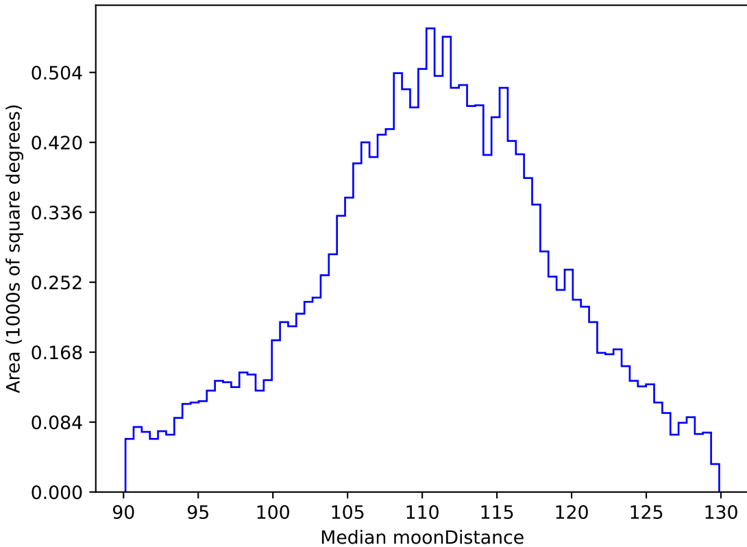
roman_v3.3_10yrs WFD r band: Median moonDistance
