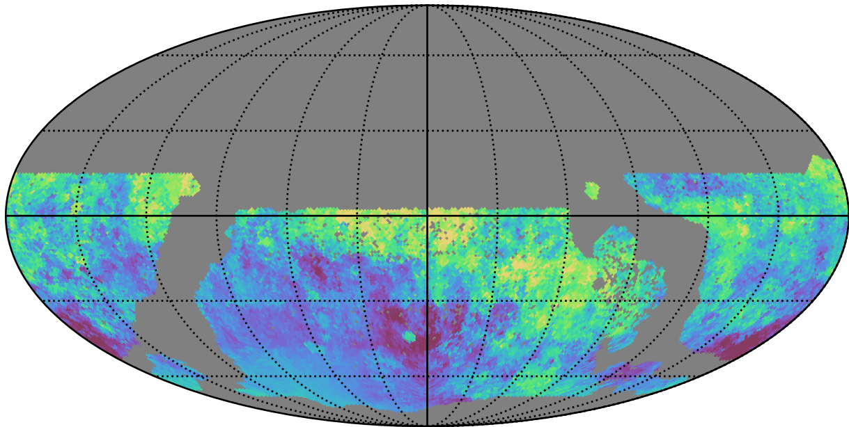
roman_v3.3_10yrs WFD i band: Median moonDistance
