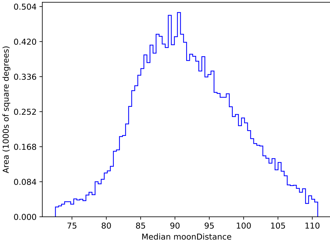
roman_v3.3_10yrs WFD i band: Median moonDistance
