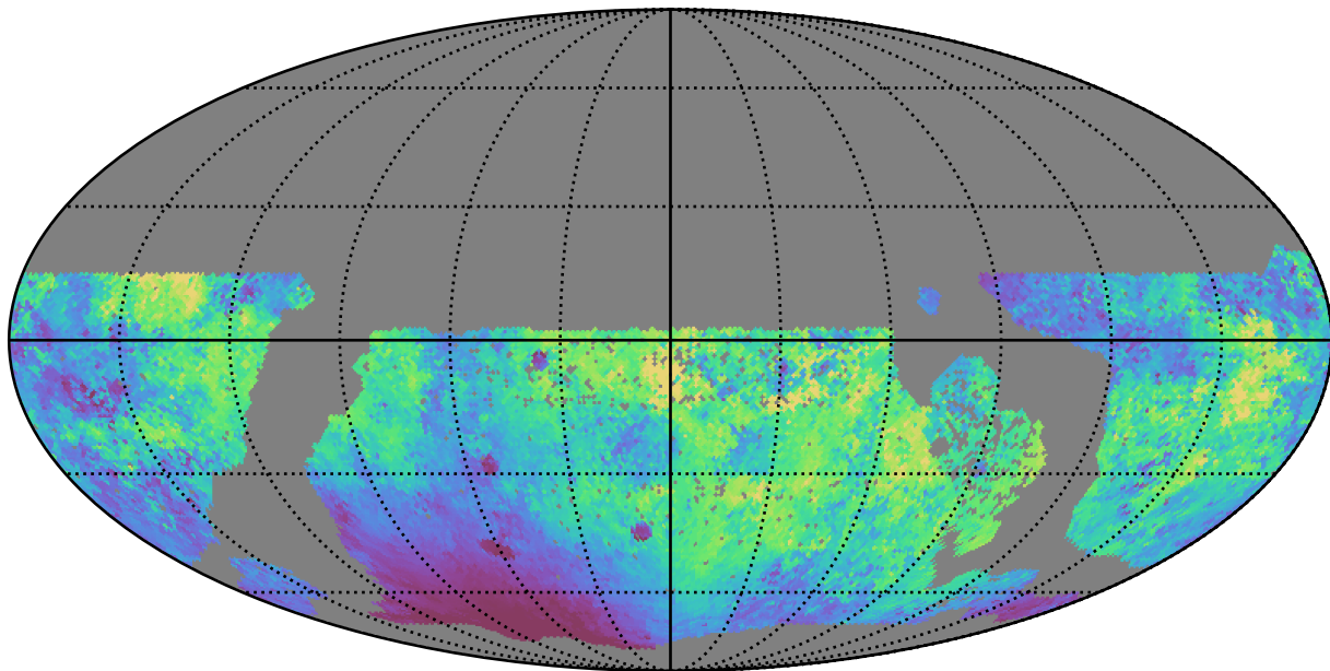
roman_v3.3_10yrs WFD g band: Median moonDistance
