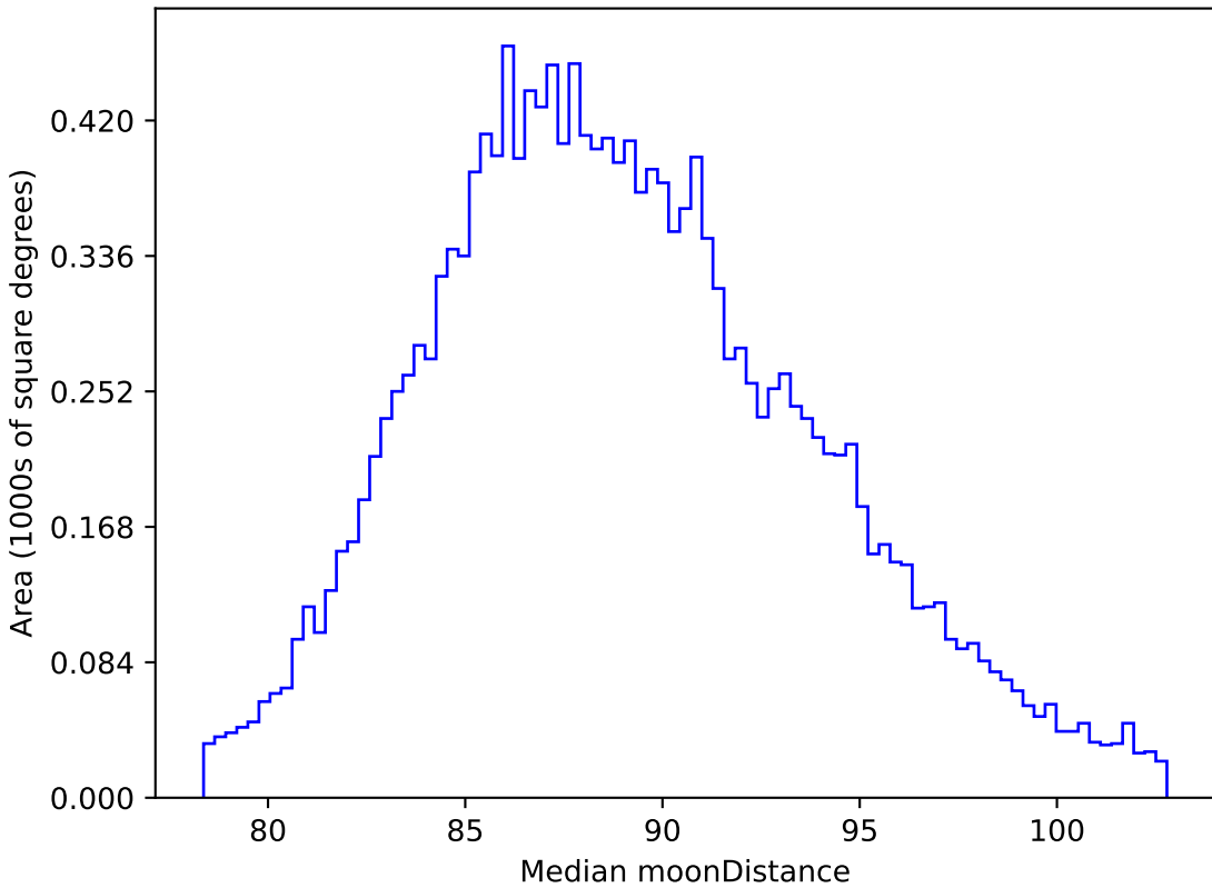
roman_v3.3_10yrs WFD all bands: Median moonDistance
