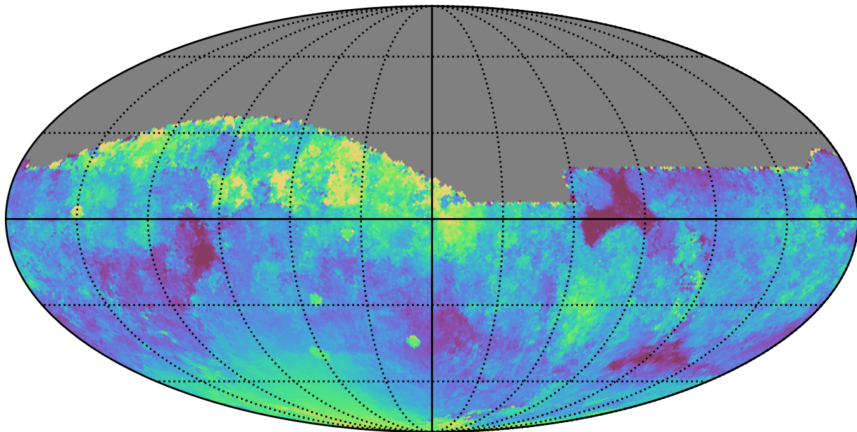
roman_v3.3_10yrs All sky z band: Median moonDistance
