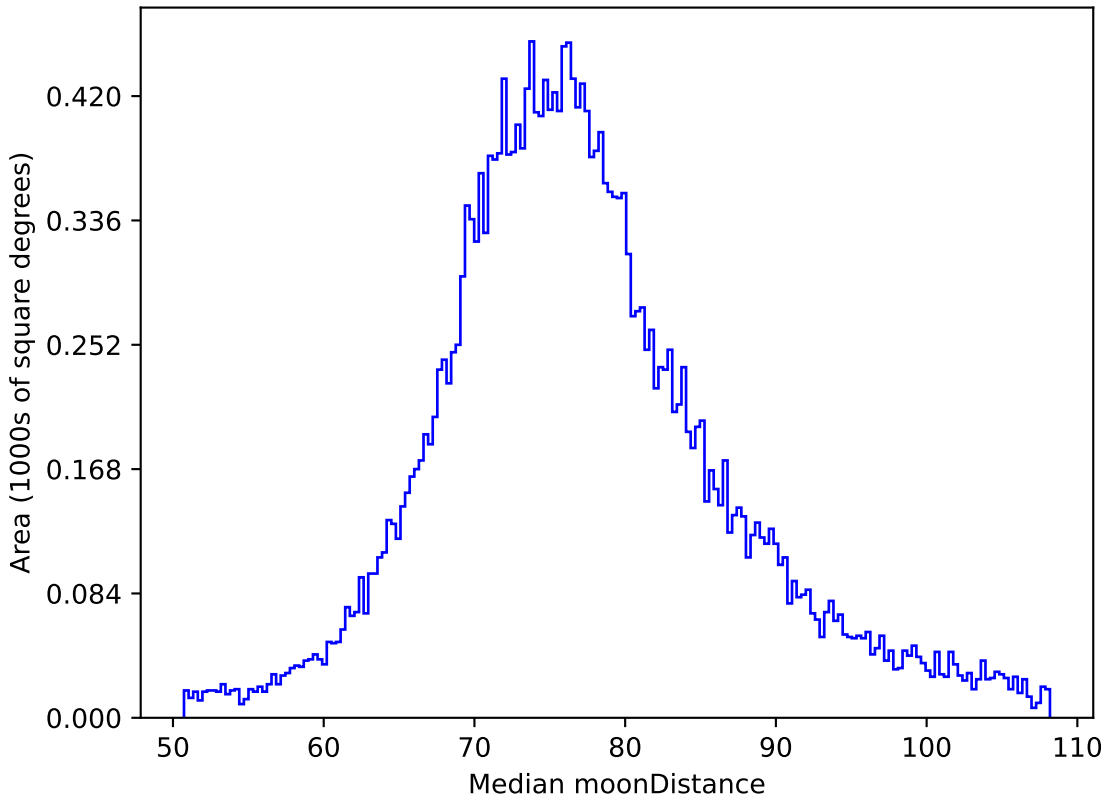
roman_v3.3_10yrs All sky z band: Median moonDistance
