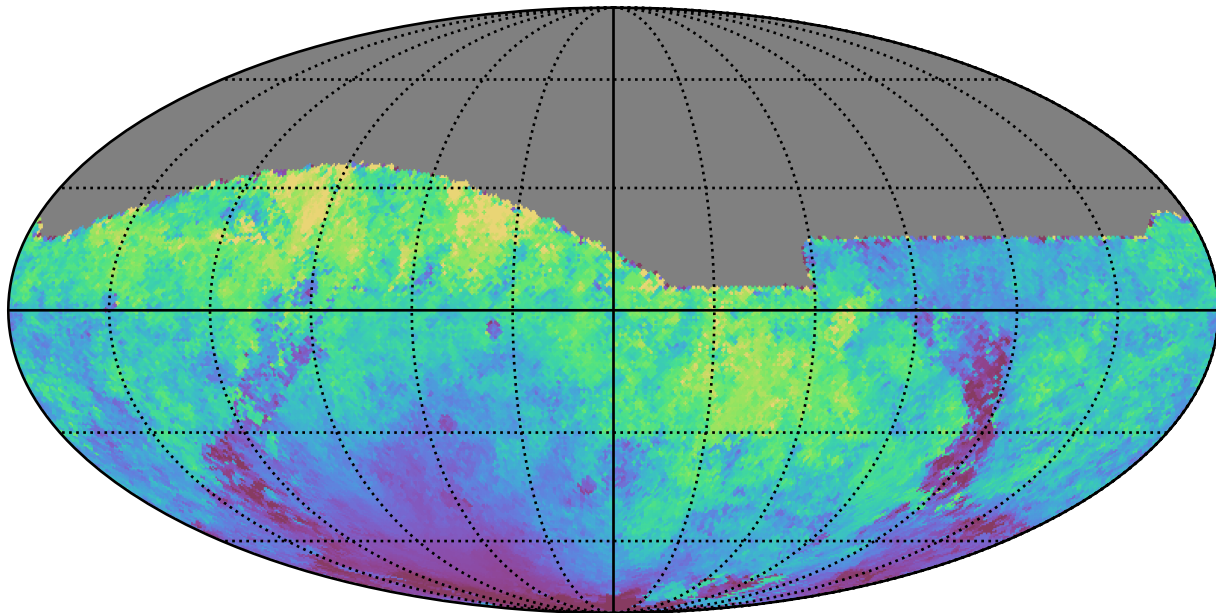
roman_v3.3_10yrs All sky r band: Median moonDistance
