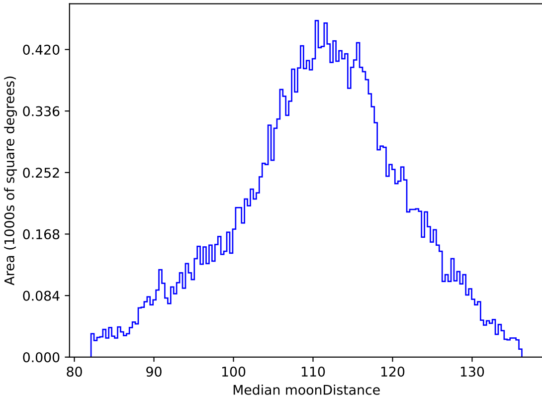
roman_v3.3_10yrs All sky r band: Median moonDistance
