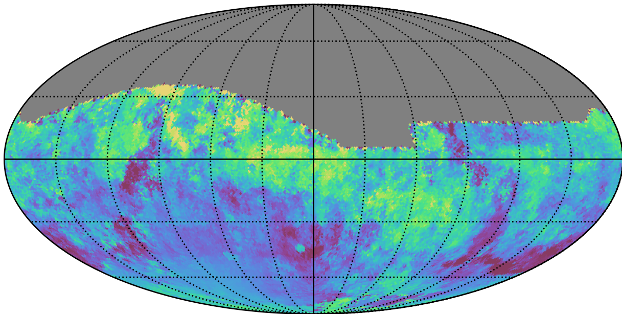
roman_v3.3_10yrs All sky i band: Median moonDistance
