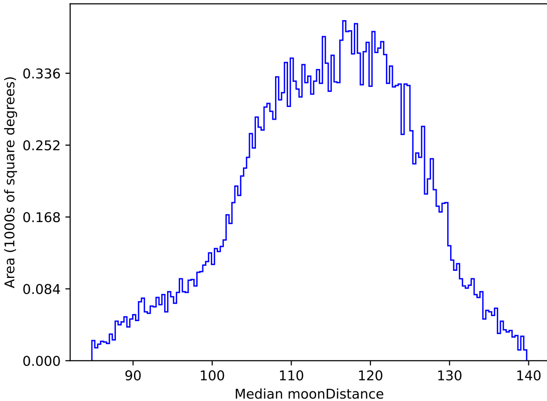
roman_v3.3_10yrs All sky g band: Median moonDistance
